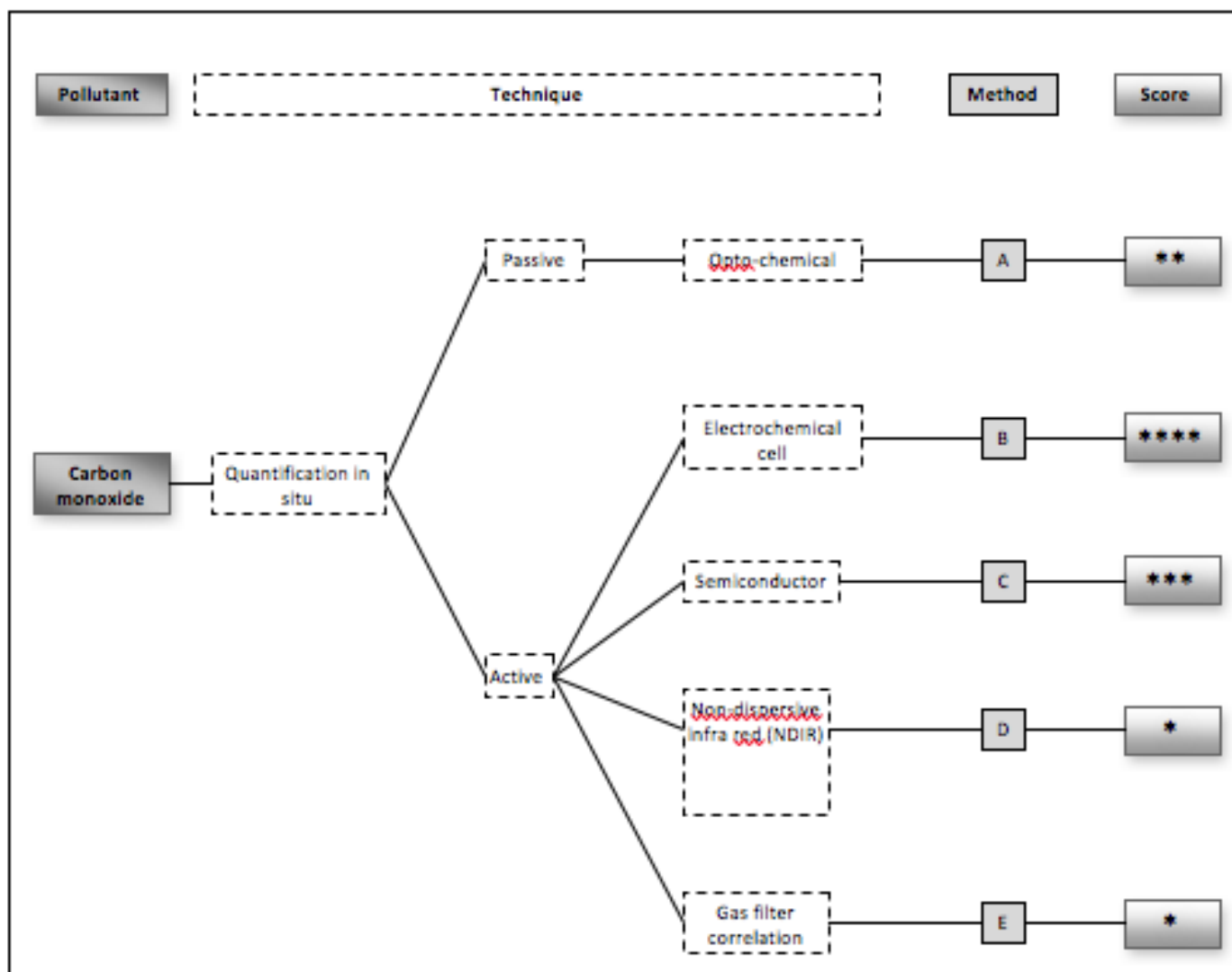
Figure 4: Measurement systems for carbon monoxide
