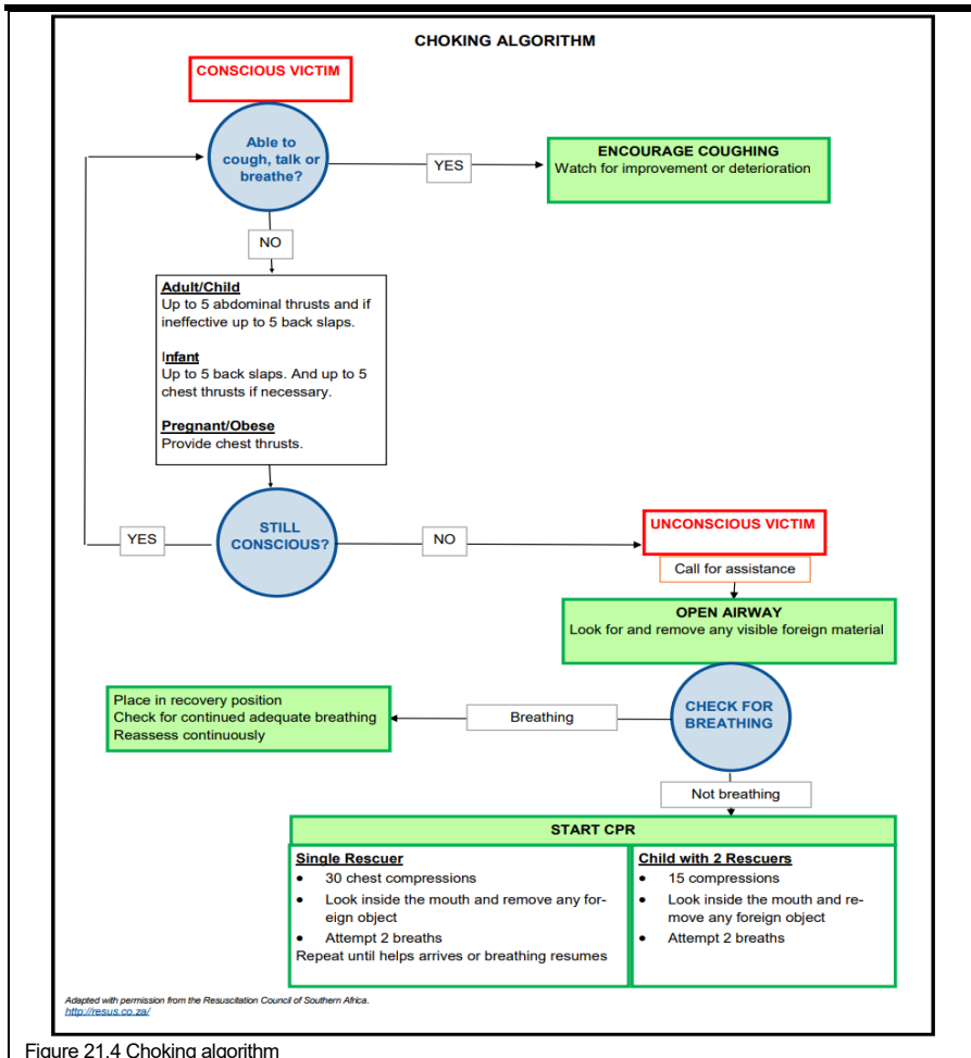
Figure 21.4 Choking algorithm
